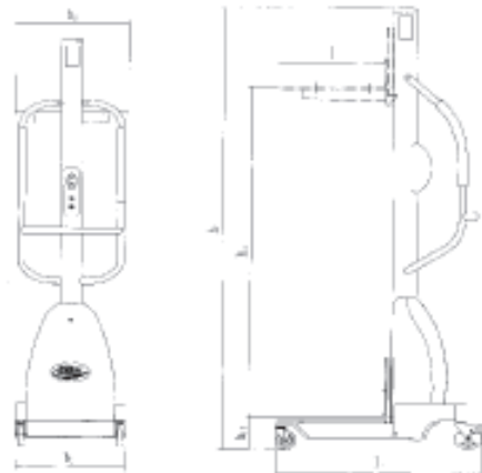
MES150B
