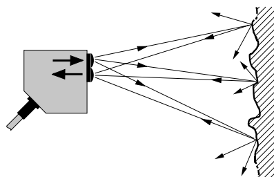
Fig. 10: Diffuse sensing
