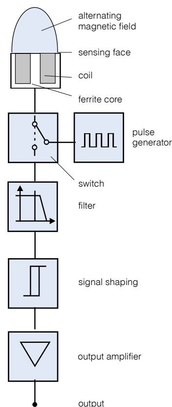
Fig. 4: Full Inox family sensors use Condect® pulse generator technology instead of an oscillator
