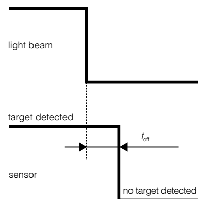
Fig. 48: Output turn-off time
